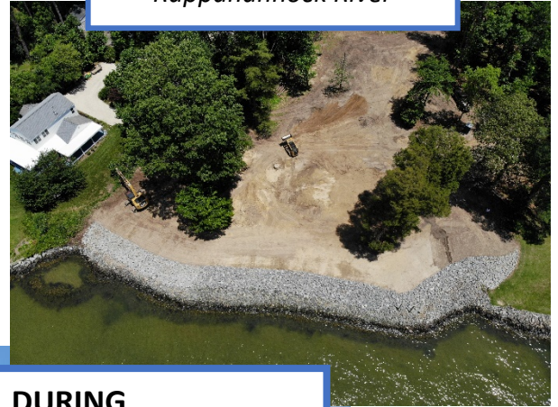
DURING After Dirt Work (Building a Slope) Rappahannock River
